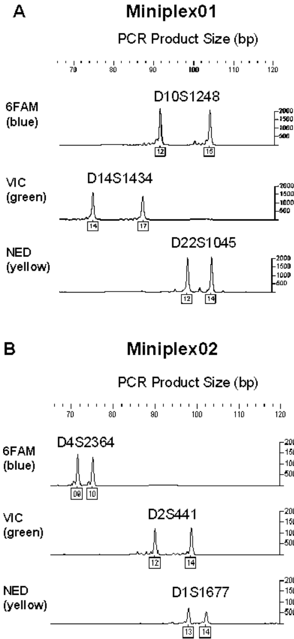
FIG. 2—Representative sample from an individual analyzed with both (A) miniplex01 and (B) miniplex02 using standard conditions for amplification (28 cycles, 1U AmpliTaq Gold polymerase, 10 \mu L PCR).
