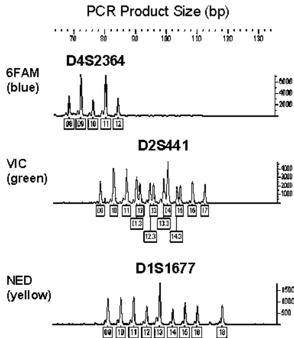
FIG. 3—MiniSTR allelic ladders for miniplex01 (top panel) and miniplex02 (bottom panel). Samples were amplified individually and electrophoretically separated on an ABI 310.
